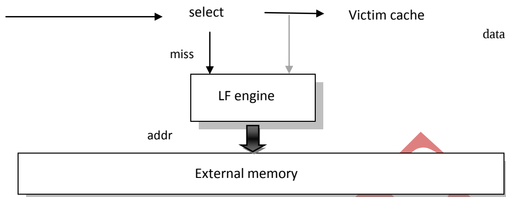
Figure 6 : Cache read request control flow with forwarding
