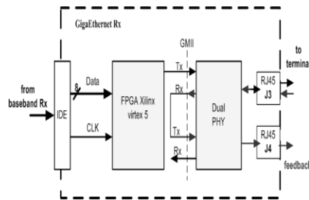
Fig. 7. 60 GHz Wireless Gigabit Ethernet receiver (Rx) Fig. 12. Receiver Gigabit Ethernet interface
