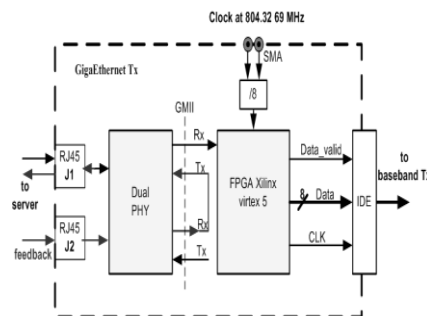
Fig. 2. Transmitter Gigabit Ethernet interface
