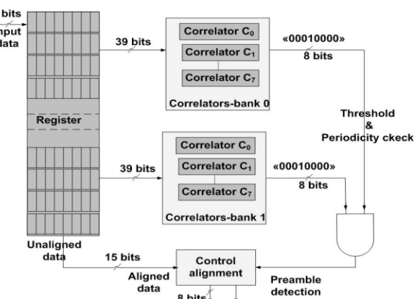
Fig. 9. Preamble detection based on periodicity and control alignment
