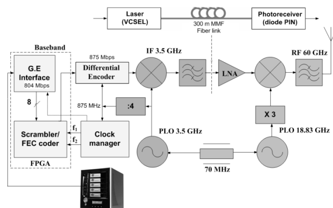
Fig. 1. 60 GHz wireless Gigabit Ethernet transmitter
