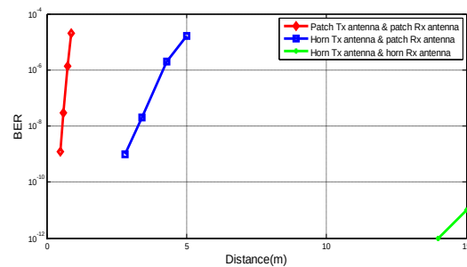
Fig. 16. BER performance at 875 Mbps (without channel coding)
