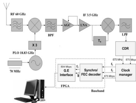
Fig. 7. 60 GHz Wireless Gigabit Ethernet receiver (Rx) Fig. 12. Receiver Gigabit Ethernet interface
