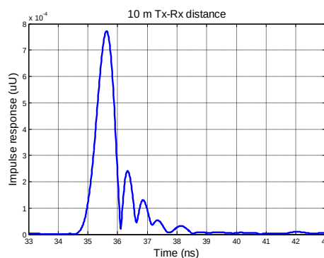
Fig. 14. Impulse response of RF blocks (using horn antennas)
