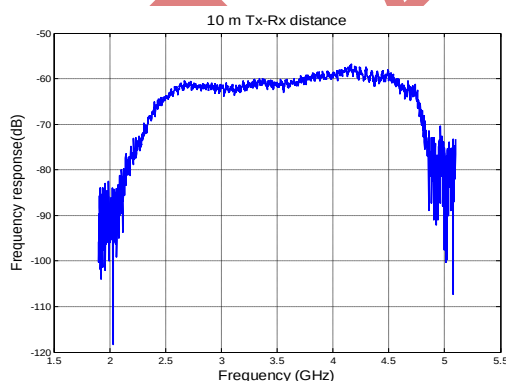
Fig. 13. Frequency response of RF Tx-Rx (with horn antennas)
