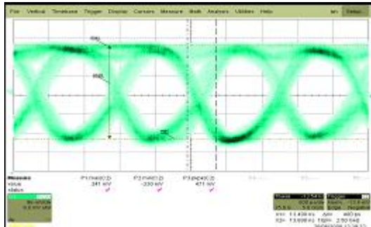
Fig. 15. Eye diagram at 875 Mbps (10 m Tx-Rx distance)
