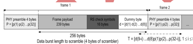
Fig. 4. Frame Structure
