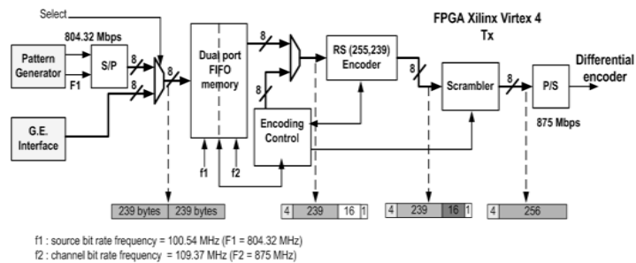
Fig. 3. BB-Tx architecture
